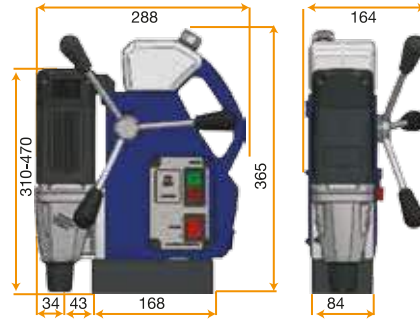
POWERTEC 32 X Magnetic Drilling Machine
