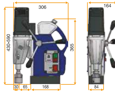
POWERTEC 50 X Magnetic Drilling Machine
