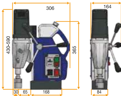
POWERTEC 50 RL X Magnetic Drilling Machine
