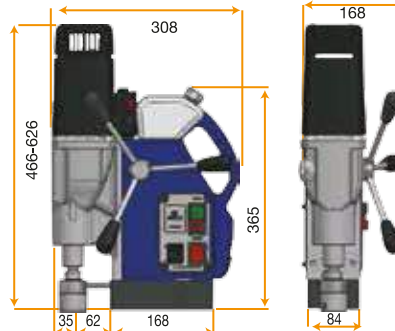
POWERTEC 60 RL X Magnetic Drilling Machine
