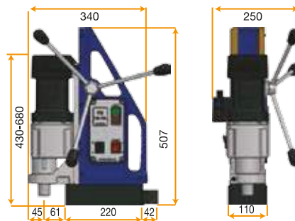
POWERTEC FE 100 RL X Magnetic Drilling Machine
