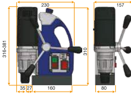
POWERTEC 30 Magnetic Drilling Machine
