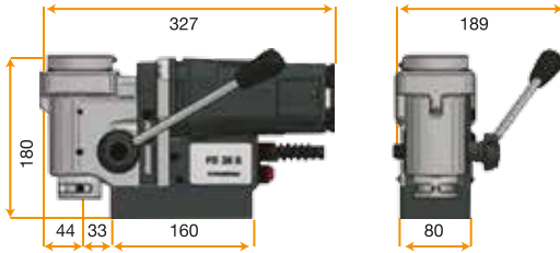
POWERTEC 36 S Magnetic Drilling Machine
